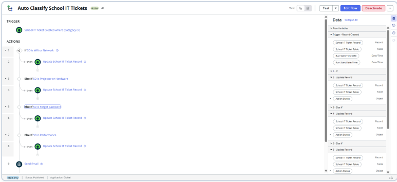
Figure 3: Published Auto Classify School IT Tickets Flow Designer workflow showing condition logic.
