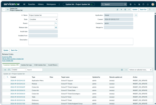
Figure 5: Completed Project Update Set containing captured customizations and XML export option.
