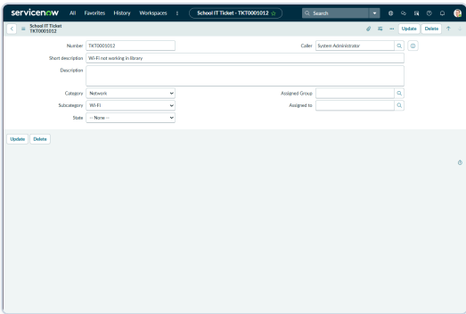
Figure 4: School IT Ticket showing the result of automatic classification (Category: Network, Subcategory: Wi-Fi).
