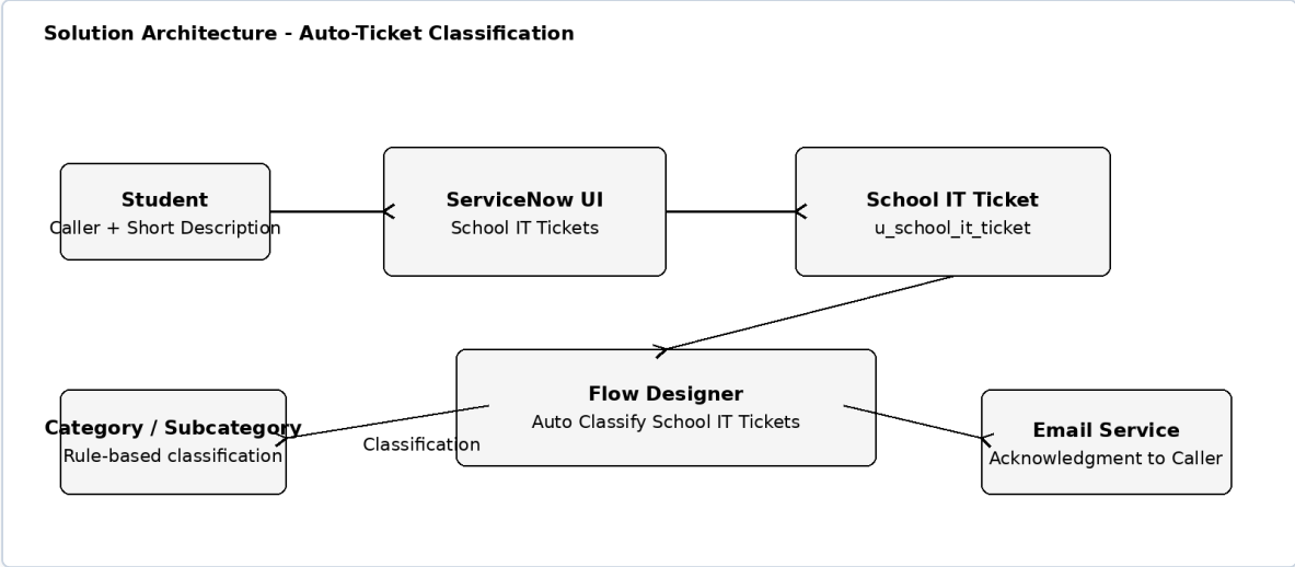
Figure 1: Solution architecture and data flow of the School IT ticket classification system.
